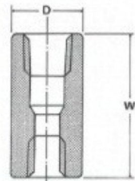
Manicotti ridotti Reducing couplings
